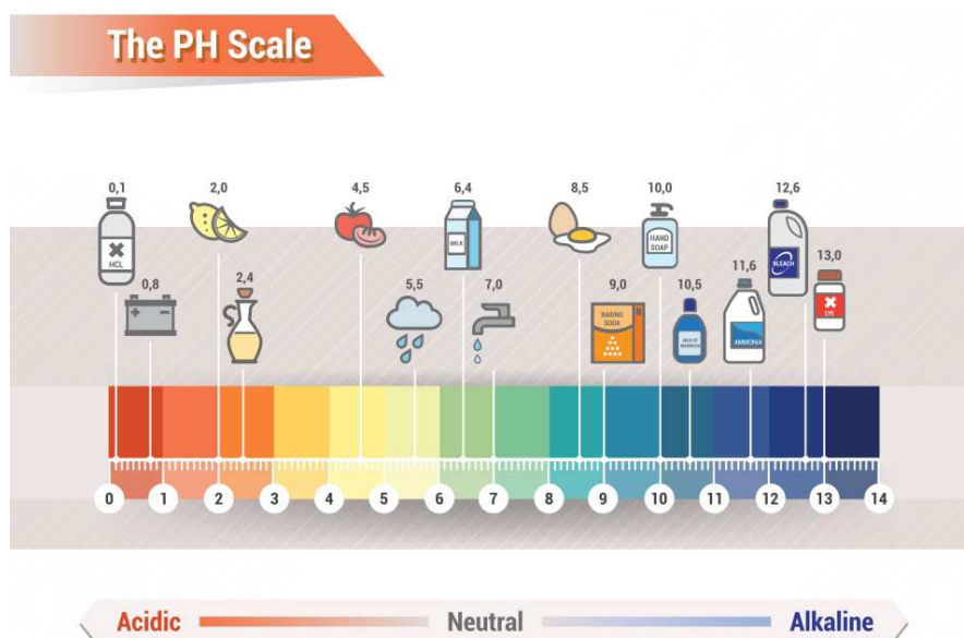
Figure 1: The pH scale
